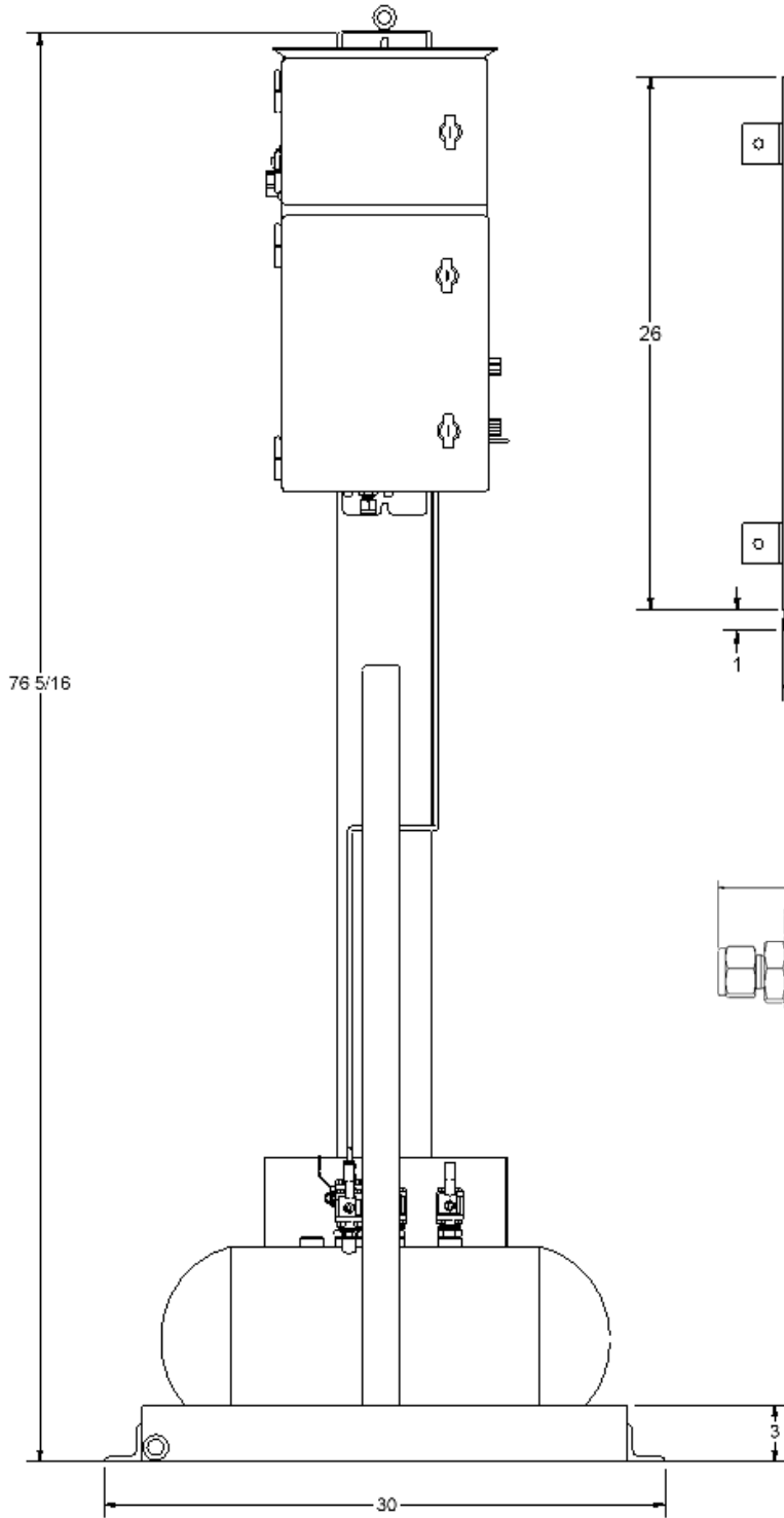
Sonic Muffler
