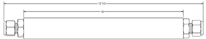
Sonic Muffler
